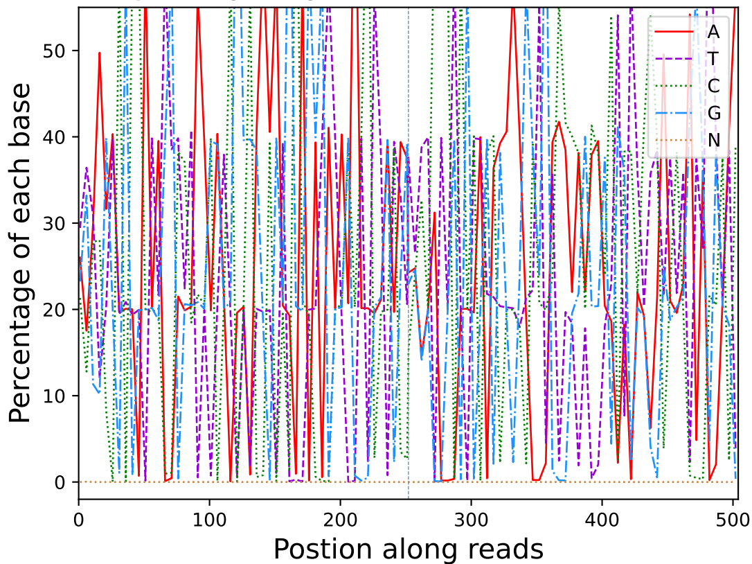
Base percentage along reads (R10614)
